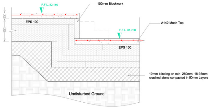
STEP DETAIL SECTION D-D Scale 1:15
