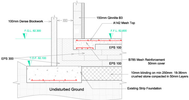
RING BEAM SECTION A-A Scale 1:15
