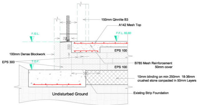
THRESHOLD DETIAL Scale 1:15
